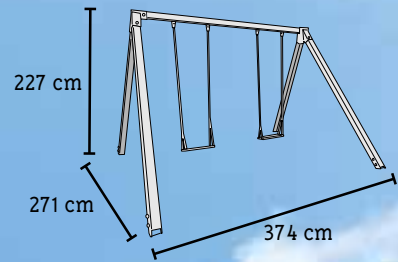
Ref: MA500105 Swing Vega Baby HORECA
